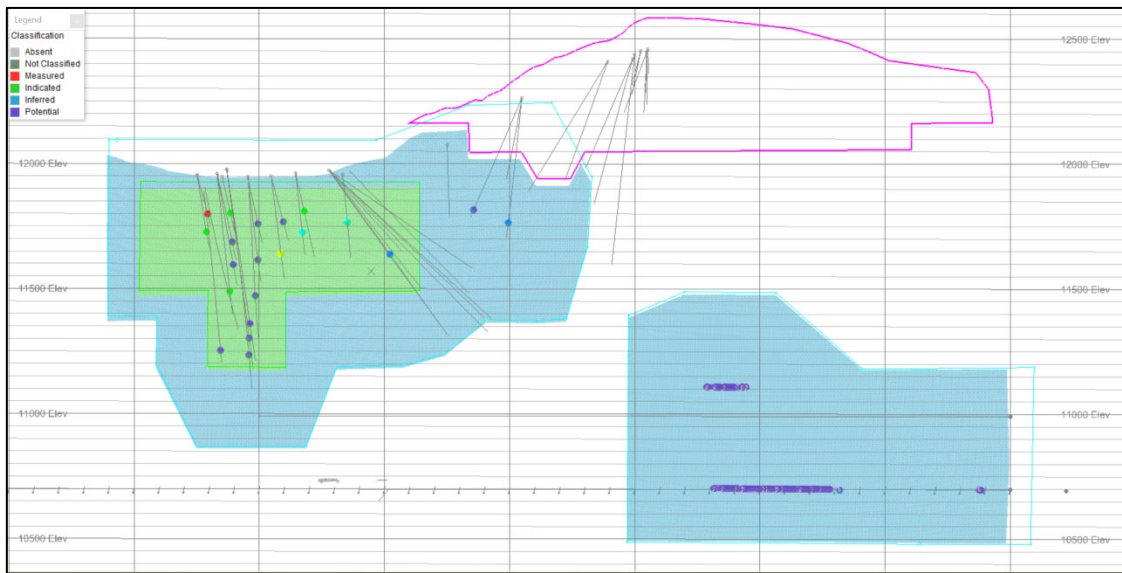
Figure 14-12: Long Section (Looking Southwest) of Terrible Vein showing Final Classification
